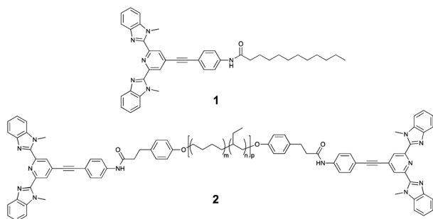
Fig. 1 Chemical structure of the low-molecular weight reference ligand 1 and the telechelic poly(ethylene-co-butylene) (PEB) macromonomer 2 (with M_n = 4200 \text{ g mol}^{-1} ; m \approx 0.36 , n \approx 0.64 , p \approx 55 ).
