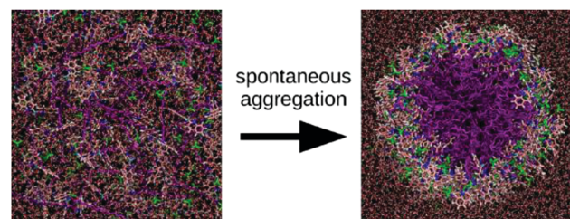
Fig. 3 Self-assembly of amphi-philic cyanine dyes into tube structure. The dye molecule is amphi-pseudocyanine, a cyanine dye with two hydrophobic tails (CH 3 and C 18 H 37 ). The dye molecules are depicted with the tails purple; the nitrogen atoms are dark blue; the aromatic carbons are pink; the linker between the aromatic rings is light blue; and hydrogens connected to aromatic carbons are white. Perchlorate counterions are shown in green. For the water molecules, oxygen atoms are red and hydrogen atoms are white. Figure adapted with permission from ref. 41. Copyright 2013 American Chemical Society.
