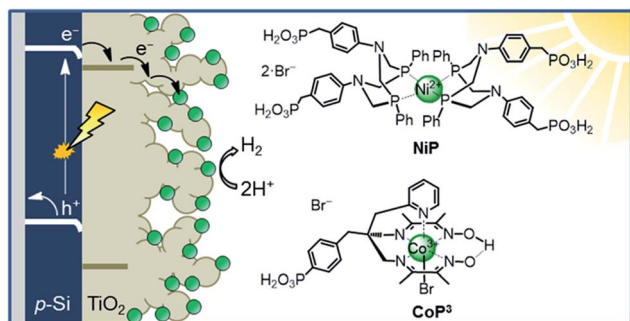
Fig. 1 Schematic diagram of PEC \text{H}_2 evolution with the \text{Si/mesoTiO}_2 /catalyst photocathode and chemical structures of the immobilised catalysts NiP and CoP 3 .
