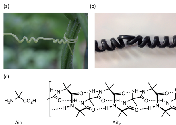
Fig. 1 Helical perversions in (a) a tendrill of the garden cucumber, Cucumis sativa , and (b) the cord of a telephone handset; (c) Aib and a portion of its 3_{10} helical homo-oligomer, shown in its right-handed screw-sense conformation.
