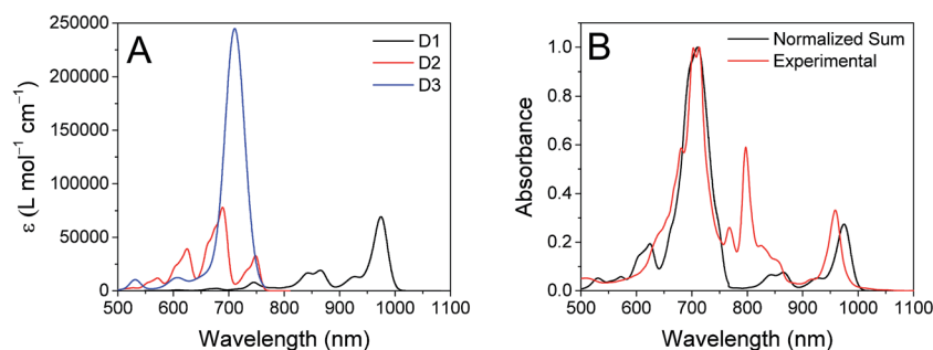
Fig. 8 Left: Calculated vibronic transitions from the ground state to the D1 (black), D2 (red) and D3 (blue) states of PDI - . Right: Sum of the three calculated vibronic spectra (black) compared to the experimentally determined spectrum of PDI - , normalized to the maximum value.
