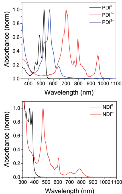
Fig. 1 Top: Spectra of PDI-Phbpy-Re-Py in the neutral (black), PDI 1- (red) and PDI 2- (blue) states. Bottom: Spectra of Phbpy-Re-PyPhNDI in the neutral (black) and NDI 1- (red) states.
