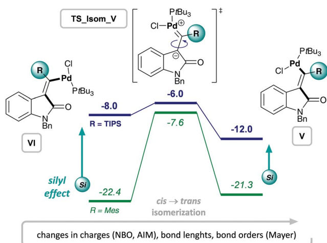
Fig. 2 Effect of alkyne substituent on Pd(II) intermediates, VI and V , and \text{cis} \rightarrow \text{trans} isomerization: analysis of charges, bond lengths and bond orders.
