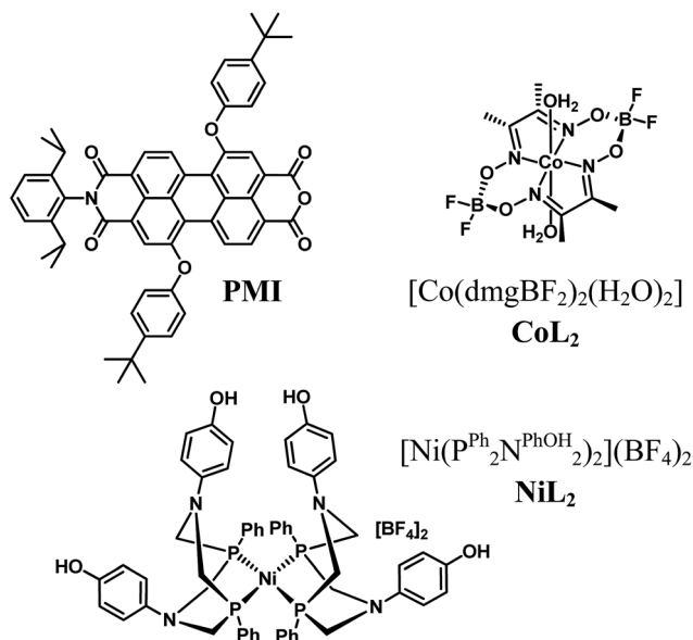
Fig. 1 Chemical structures of the PMI photosensitizer and the \text{H}_2 evolution catalysts.
