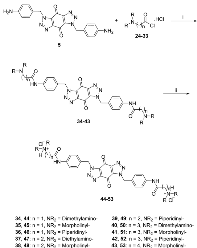
Scheme 3 General synthetic route for the target ligands 44–53. Reagents and conditions: (i) (a) pyridine, DMF, rt, 16 h, (b) \text{NaHCO}_3(\text{aq}) , 38–90%; (ii) 0.5 M \text{HCl}/\text{CH}_3\text{OH} , rt, 4 h, 65–95%.
