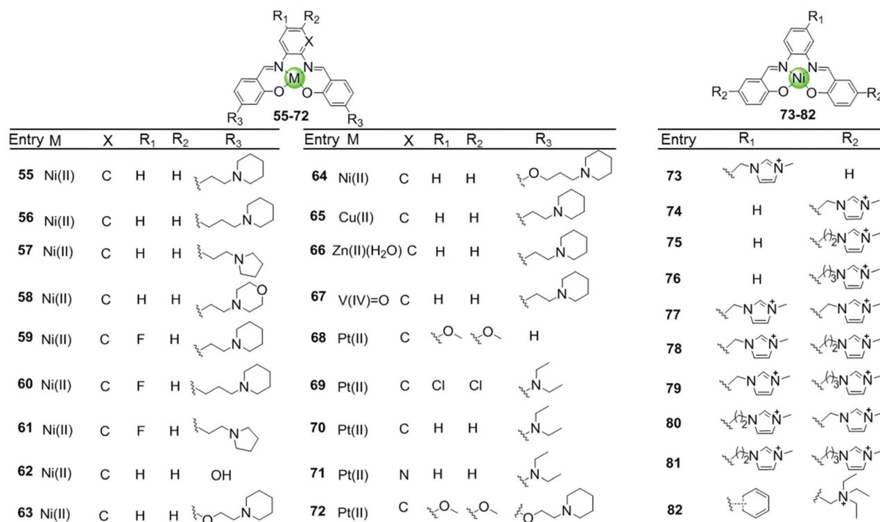
Fig. 8 Metallosalphens with various side arms reported as G4-ligands. 66–73
