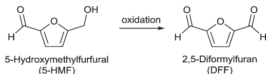
Scheme 7 Conversion of 5-HMF to 2,5-diformylfuran (DFF).
