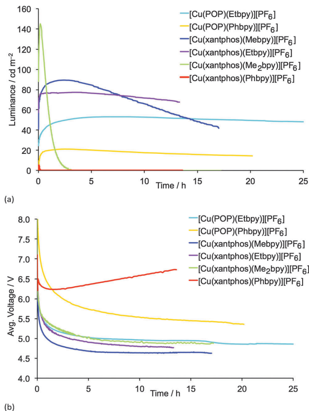
Fig. 10 Luminance (a) and average voltage (b) for ITO/PEDOT:PSS/[Cu(P ^ P)(N ^ N)][PF 6 ]:[Emim][PF 6 ] 4:1 molar ratio/Al LECs measured using a pulsed current driving (average current density 50 A m -2 , 1 kHz, 50% duty cycle, block wave). [Emim][PF 6 ] = 1-ethyl-3-methylimidazolium hexafluoridophosphate.
