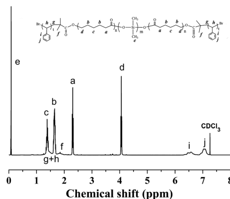
Fig. 4 1 H NMR spectrum of the PS- b -PCL- b -PDMS- b -PCL- b -PS pentablock copolymer.
