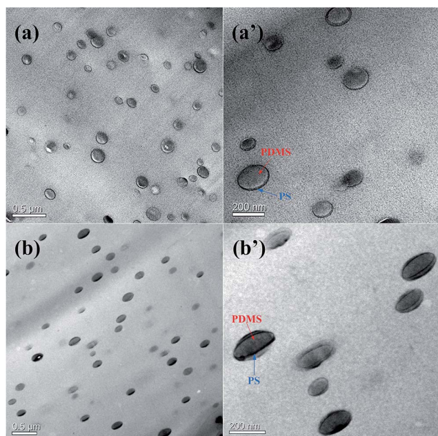
Fig. 5 The TEM images of the epoxy thermosets containing 10 wt% (a and a') and 20 wt% (b and b') PS- b -PCL- b -PDMS- b -PCL- b -PS pentablock copolymer.
