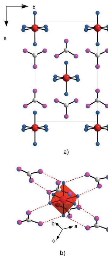
Fig. 23 Representation of the non-centrosymmetric structure of [\text{C}(\text{NH}_2)_3]_2[\text{TiF}_6] ; (a) in the ab plane; and (b) showing the \text{F} \cdots \text{H} bonds. Adapted from ref. 110 (Copyright © 2011 Elsevier Inc).
