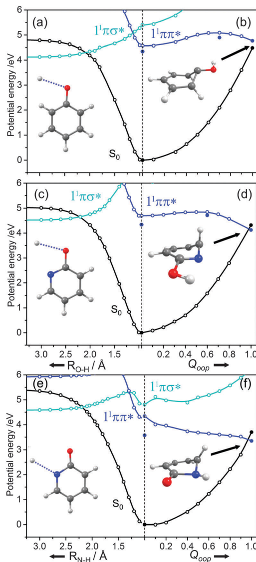
Fig. 8 Potential energy profiles for the ground and lowest singlet excited states along, respectively, R_{X-H} ( X = O, N ) and Q_{oop} for phenol ((a) and (b)), 2-hydroxypyridine ((c) and (d)) and 2-pyridone ((e) and (f)). Filled points define the energies of the optimised critical structures ( i.e. the S_0 and 1\pi\pi^* minima, the S_0/1\pi\pi^* CI and the TS on the 1\pi\pi^* potential leading to the prefulvenic S_0/1\pi\pi^* CI). The structures in each panel illustrate, respectively, the X–H bond dissociation coordinate and the optimised geometry at the prefulvenic S_0/1\pi\pi^* CI.
