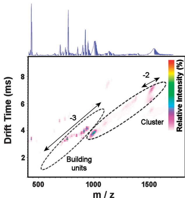
Fig. 3 ESI-IMS-MS of \{\text{Mo}_{16}\} 1 in MeOH. Relative intensity (cf. highest peak) is shown on a linear scale (coloured scale, inset); samples of isotope patterns (inset) were obtained in resolution mode; see ESI† for details.
