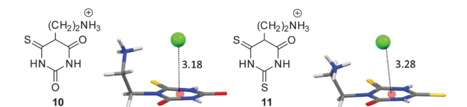
Fig. 6 Molecular structures, quadrupole moments and molecular polarizabilities of selected thio cyanuric acid derivatives and their corresponding anion- \pi complexes with chloride (including the calculated interaction energies and equilibrium distances). Additionally, the ion pairs of the ethylene ammonium-substituted chloride salts of the thio- (10) and dithiocyanuric acids (11) are shown as observed in the solid state. 19c
