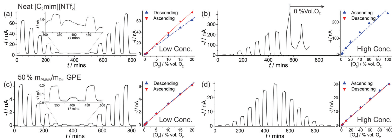
Fig. 4 Long-term chronoamperometry (LTCA) at different O_2 gas concentrations in (a, b) neat [C_2mim][NTf_2] and (c, d) 50% m_{PMMMA}/m_{Tot} . PMMA- [C_2mim][NTf_2] mixture. The gas flow was alternated between 100 vol% N_2 and varying O_2 concentrations: "low concentration" (a, c) 20, 15, 10, 5, 1, 0.5, 0.1, 0.5, 1, 5, 10, 15, 20 vol% and "high concentration" (b, d) 1.1, 2.7, 10, 20, 40, 60, 80, 100 vol% and (d) 1.1, 2.7, 10, 20, 40, 60, 80, 100, 80, 60, 40, 20, 10, 2.7, 1.1 vol% O_2 . Background subtracted current vs. concentration plots are shown on the right, along with the lines of best fit from the "descending" and "ascending" data sets. The equations of the line of best-fit, R^2 value, and LODs are given in Table 2.
