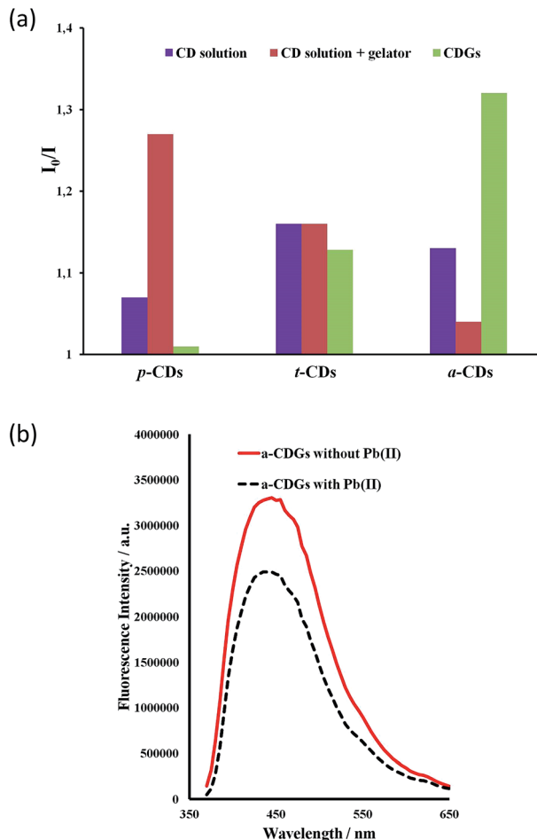
Fig. 8 (a) Photoluminescent response to 10 \text{ µg mL}^{-1} of \text{Pb}^{2+} to CD solutions, CD-containing hydrogels (CDGs) and CD solutions in the presence of dissolved gelator ( 1 \text{ mg mL}^{-1} , \lambda_{\text{ex}} = 370 \text{ nm} ) and for 1 wt% CD-gels with 1a at the same CD concentration. (b) Fluorescence emission spectra for a-CD gel samples with and without \text{Pb}^{2+} ( 10 \text{ µg mL}^{-1} ).
