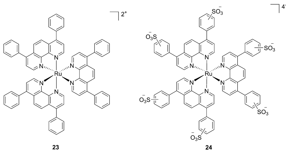
Fig. 20 Structures of the Ph 2 phen complexes 23 and 24 with different charges investigated by Glazer and co-workers. 61
