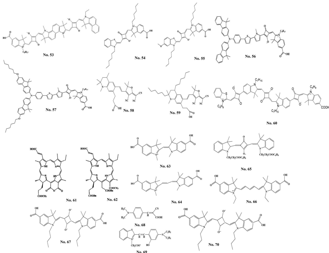
Fig. 7 The structure of metal-free NIR organic sensitizers.
