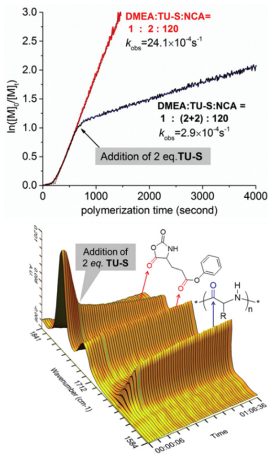
Fig. 6 \ln([\text{NCA}]_0/[\text{NCA}]_t) vs. time for the ROP of Glu-NCA initiated by DMEA/TU-S ( [\text{M}] = 0.19 \text{ M} , [\text{Glu-NCA}]/[\text{TU-S}]/[\text{DMEA}] = 120/(2 + 2)/1 , 25 °C, \text{CH}_2\text{Cl}_2 ) and corresponding 3D kinetic behavior profile from in situ IR (the sampling interval of in situ IR is 10 seconds).
