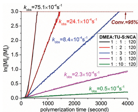
Fig. 4 Kinetics of the ROP of Glu-NCA promoted by DMEA/TU-S ( [\text{M}] = 0.19 \text{ M} , [\text{Glu-NCA}]/[\text{DMEA}] = 120 , [\text{TU-S}]/[\text{DMEA}] = 1, 2, 3, 5 , and 10 , 25 °C, \text{CH}_2\text{Cl}_2 , the automatic sampling interval of in situ IR is 10 seconds).
