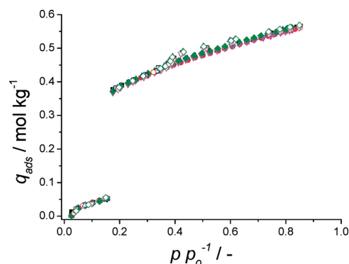
Fig. 4 Repeated \text{H}_2\text{O} adsorption isotherms at 298 K of CAU-10-H supported on a metallic aluminium plate. First (■), second (●), third (▲), fourth (▼) and fifth (◆) measurements. Closed symbols depict adsorption, open desorption. Loading is presented as per total mass of sample (Al substrate + CAU-10-H).
