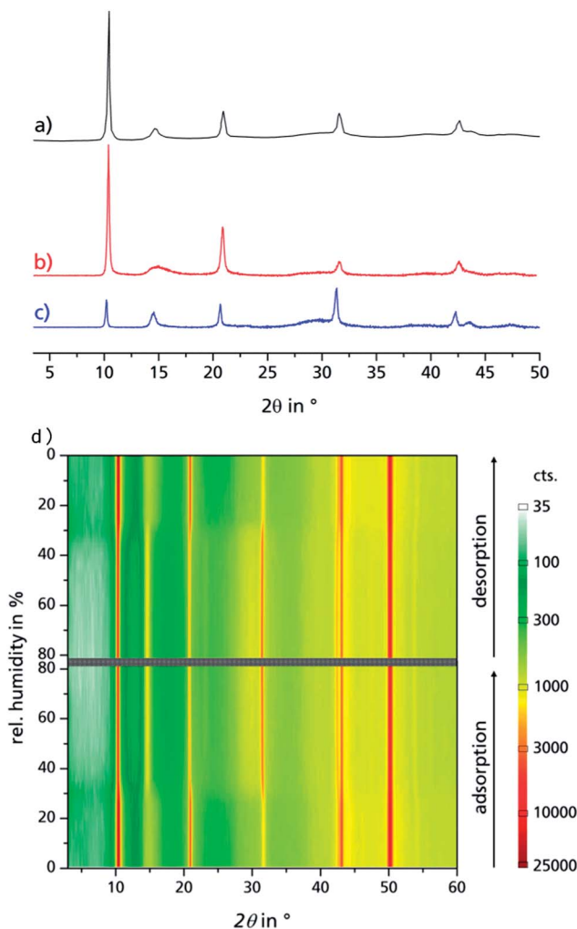
Fig. 2 PXRD of bulk \mu\text{p-AF} as extracted from patent literature (a), dried \mu\text{p-AF} (stored at 120^\circ\text{C} under vacuum for 24 h (b)) and hydrated \mu\text{p-AF} (stored under 100% water vapour atmosphere overnight, (c)). (d) Reversible structural transition observed by in situ PXRD in a humidity chamber at 313 K. See Fig. S5 in the ESI† for the individual diffractograms.
