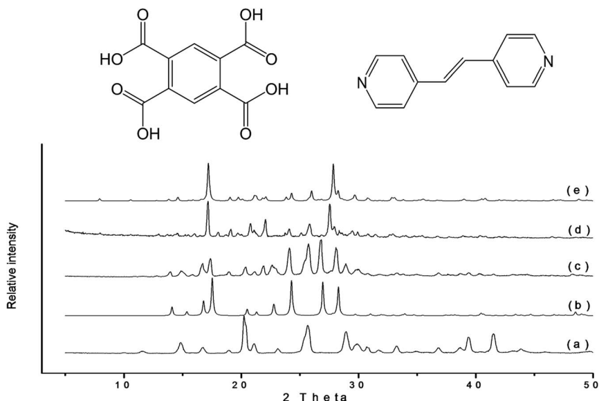
Fig. 15 Demonstration of the enhanced kinetics of cocystal formation upon addition of a few drops of methanol to the grinding jar. PXRD patterns for (a) tetracarboxylic acid, (b) bipyridyl, (c) outcome of neat grinding for 60 minutes (as the sum of the reactants), (d) the product obtained when a few drops of methanol are added and (e) the simulated pattern for the cocystal.
