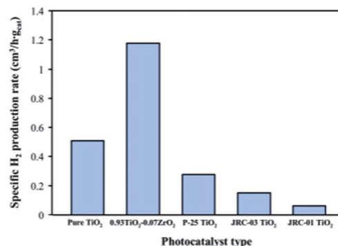
Fig. 15 The effect of the photocatalyst type on the specific \text{H}_2 production rate over the synthesised mesoporous-assembled pure \text{TiO}_2 and 0.93\text{TiO}_2\text{-}0.07\text{ZrO}_2 mixed oxide photocatalysts calcined at 500^\circ\text{C} when compared to commercial \text{TiO}_2 photocatalysts (P25, JRC-01 Ishihara Sangyo Co., JRC-03 Ishihara Sangyo Co.).
