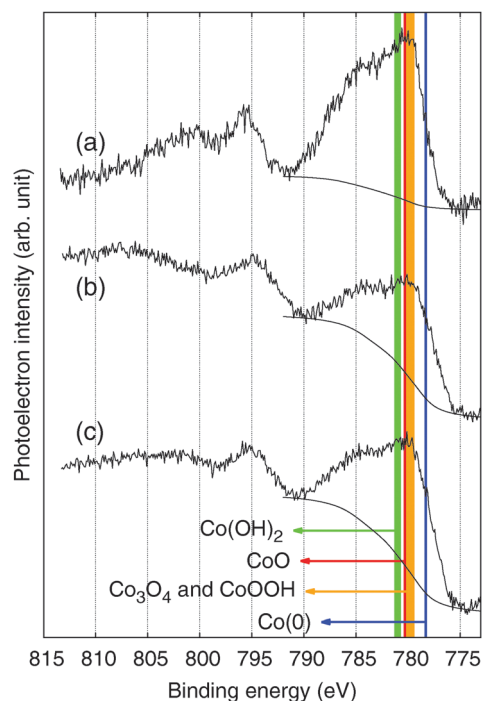
Fig. 7 XPS spectra in the Co 2p region for the (a) ball-milled CoFe-CNFs, (b) CoFe-CNFs, and (c) Co-CNFs.
