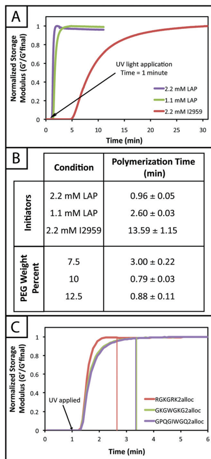
Fig. 2 In situ polymerization of PEG hydrogels with different photoinitiators. (A) Hydrogels (10 wt% with respect to PEG) were polymerized in situ on a rheometer to monitor gel formation over time using various initiator conditions. After 1 minute on the rheometer, UV light (10 mW cm -2 , 365 nm) was applied to samples. The storage moduli of gels polymerized using 1.1 and 2.2 mM LAP initiator begin to increase within 30 seconds after light application and finish forming in approximately 1–3 minutes (modulus levels off). Gels polymerized using 2.2 mM I2959 begin to form 4 minutes after UV light application and reach complete formation in approximately 13–14 minutes of exposure. The rapid polymerizations observed for the LAP initiator are relevant for cell culture applications. Representative data for each condition is shown here. (B) Complete polymerization, defined here as the point where the change in modulus between consecutive data points is less than 0.1%, was determined for various initiator and monomer concentrations. As shown in (A), the LAP initiator exhibits the most rapid polymerization, with times of 0.96 ± 0.05 and 2.60 ± 0.03 minutes for 2.2 and 1.1 mM LAP, respectively. Complete polymerization for I2959, at the highest concentration compared to LAP (2.2 mM), occurs in 13.59 ± 1.15 minutes. Using 2.2 mM LAP, hydrogels from various initial monomer concentrations (7.5, 10, and 12.5 wt% with respect to PEG) were polymerized. The 7.5 wt% condition exhibited the slowest polymerization rate of 3.00 ± 0.22 minutes due to fewer functional groups that are available to react. The 10 and 12.5 wt% gels polymerized in 0.79 ± 0.03 and 0.88 ± 0.11 minutes as the number of functional groups in solution is higher at the start of polymerization. (C) Hydrogels were polymerized with different alloc-modified peptides to evaluate any effect of peptide chemistry on polymerization rate. The less charged GKGWKG2alloc and GPQGIWGQ2alloc peptides take 40 seconds longer to polymerize than the charged RGKGRK2alloc peptide, although this is not as significant as the effects of weight percent and the type and concentration of initiator on polymerization time.
