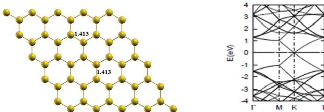
Fig. 2 The optimized geometry and band structure of a pure graphene sheet. The bond length is in Å. The Fermi level in the band structure is set to zero.
