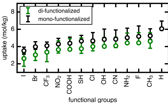
Figure 5. Range of methane uptake (in mol/kg) at 298 K and 65 bar in UiO-66 with mono- and di-functionalized BDC linkers. 13 different functional groups were studied. Circles represent the uptakes of methane in structures with unrotated linkers and whiskers indicate maximum and minimum values. The functional groups are ordered on the x-axis by increasing uptake of corresponding mono-functionalized structures with unrotated linkers from left to right.
