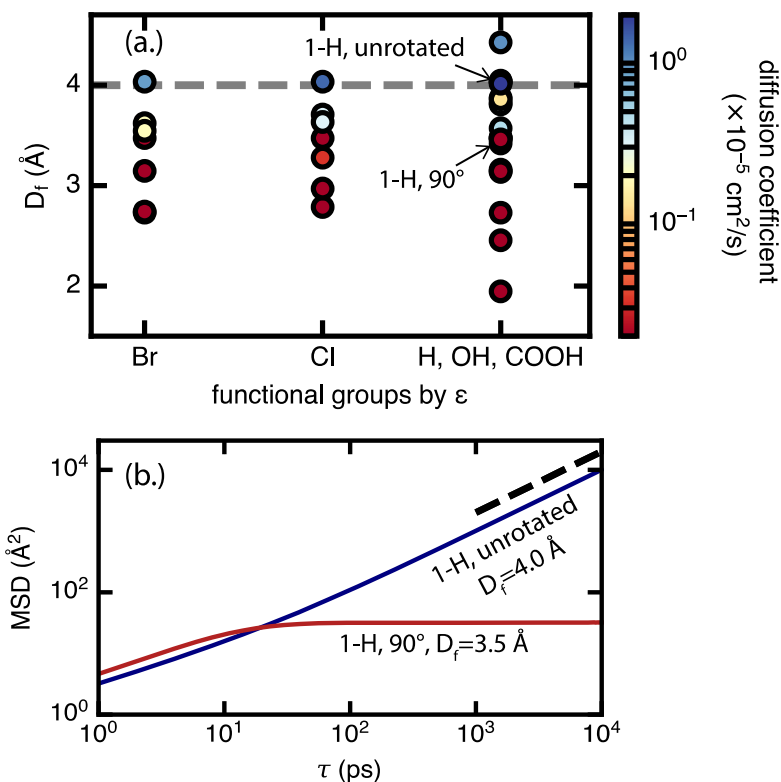
Figure 8. (a.) Methane diffusion coefficient (in \text{cm}^2/\text{s} ) at 298 K and 65 bar, labeled by color of the symbols shown, in mono-functionalized derivatives of UiO-66 as a function of two features – minimum pore size D_f in \text{\AA} (y-axis) and the Lennard-Jones potential well depth parameter \epsilon (x-axis) of the functional group atom with the highest bond path from the terminal BDC carbon. The functional groups on the x-axis are ordered by decreasing \epsilon , where functional groups that have the same \epsilon are given the same x-axis position. Rotamers that result in sub-diffusive methane are represented by the darkest shade of red on the color scale. The dashed gray line represents a ‘critical’ pore size of \sim 4 \text{ \AA} where the diffusion coefficient of methane changes from 0 to >1 \times 10^{-5} \text{ cm}^2/\text{s} , characterizing a transition from the sub-diffusive regime to Fickian diffusive regime. (b.) MSD ( \text{\AA}^2 ) of methane over lag time \tau (ps) in two example UiO-66 derivatives. The first is the unfunctionalized (1-H) unrotated rotamer with D_f = 4.0 \text{ \AA} (equal than the critical pore size) and allows for methane diffusion in the Fickian regime (black dotted line slope representative of Fickian diffusive regime). The second is the unfunctionalized (1-H) 90° rotamer with a D_f = 3.5 \text{ \AA} (below the critical pore size) and results in sub-diffusive methane. Lines represent the average of 3 independent 30 ns trajectories.
