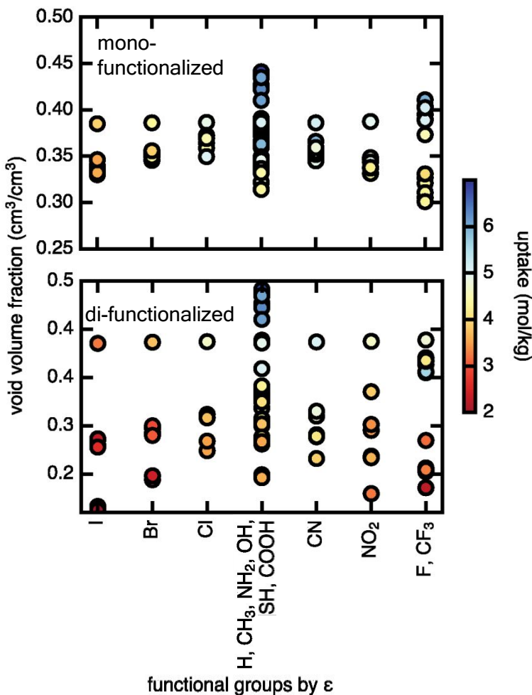
Figure 7. Methane uptake (in mol/kg) at 298 K and 65 bar, labeled by color of the symbols shown, in mono- and di-functionalized derivatives of UiO-66 as a function of two features: void volume fraction in cm 3 /cm 3 (y-axis) and the Lennard-Jones potential well depth parameter \epsilon (x-axis) of the functional group atom with the highest bond path from the terminal BDC carbon. The functional groups on the x-axis are ordered by decreasing \epsilon from left to right, and functional groups that have the same \epsilon are given the same x-axis position.
