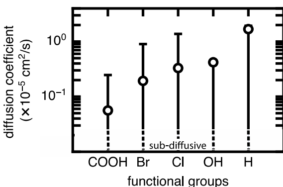
Figure 6. Range of methane diffusion coefficients (in cm 2 /s) at 298 K and 65 bar in UiO-66 with mono-functionalized BDC linkers. 5 different functional groups were studied. Circles represent diffusion coefficients of methane in structures with unrotated linkers, and whiskers indicate maximum and minimum values. The minimum values for all functional groups studied are in the sub-diffusive regime as indicated by the dotted lines. No discrete diffusion coefficient is obtained for this regime. The functional groups are ordered on the x-axis by increasing diffusion coefficient of corresponding mono-functionalized structures with unrotated linkers from left to right.
