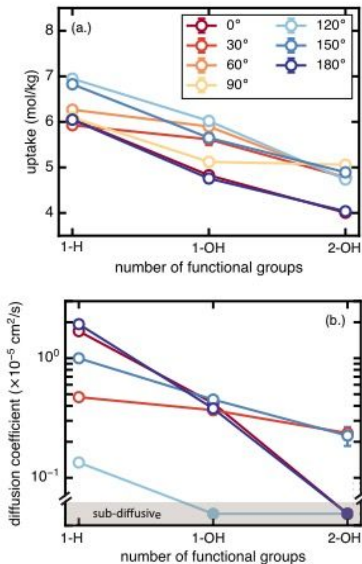
Figure 4. (a.) Methane uptake (in mol/kg) and (b.) diffusion coefficient (in \text{cm}^2/\text{s} ) at 298 K and 65 bar in UiO-66 functionalized with 0 (1-H), 1 (1-OH), or 2 (2-OH) functional groups, representing progressively larger sizes of functionalization. The OH group is chosen as a representative functional group, and the 1-H functional group is the unfunctionalized UiO-66. Error bars are obtained from the standard deviation from 5 block averages for uptake and 3 independent simulations for diffusion coefficient, both with a 95% confidence interval. Filled circles in (b.) indicate diffusion in the sub-diffusive regime. No discrete diffusion coefficients are calculated for this regime. Methane diffusion for the 90° rotamer is not shown since it displays sub-diffusive behavior for all 3 degrees of functionalization.
