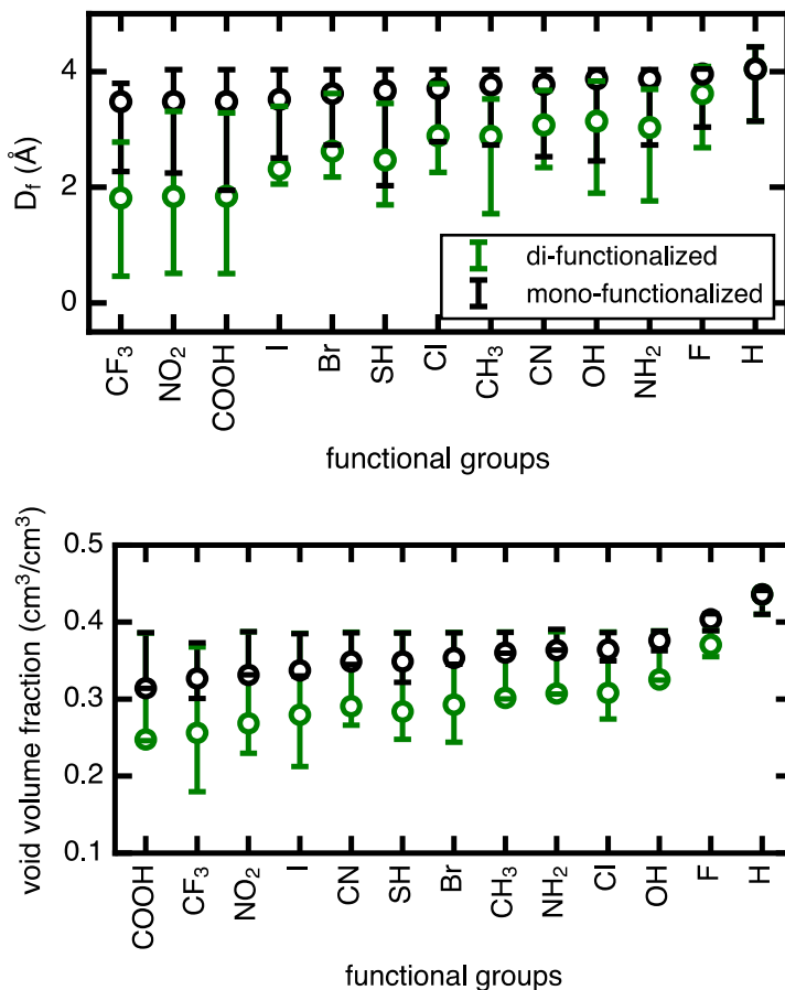
Figure 3. Range of minimum pore size D_f (in Å) and void volume fraction (in \text{cm}^3/\text{cm}^3 ) features obtained by Zeo++. The span of both features is obtained by sampling the angular rotamers of the BDC linker in all 13 (mono- and di-functionalized) functional group derivatives of UiO-66. Circles correspond to D_f and void volume fraction of structures with unrotated linkers, and whiskers indicate maximum and minimum values. The functional groups are ordered on the x-axis left to right by increasing values for mono-functionalized structures with unrotated linkers of D_f and void volume fraction in the top and bottom plots, respectively.
