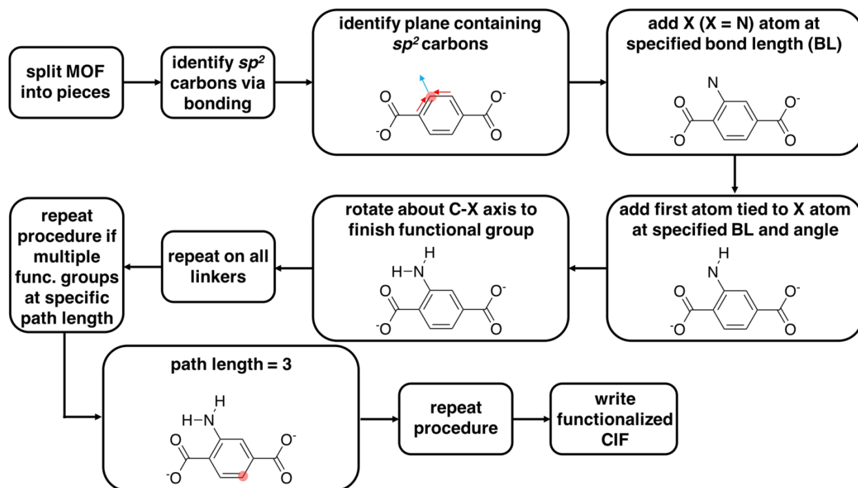
Figure 1. Flowchart for MOF functionalization procedure. After the code identifies the linkers, sp^2 carbon atoms containing C–H bonds are identified. The plane of the functionalized carbon (red circle) is identified, and the direction of the functionalization (blue vector) is identified by the two adjacent carbons (red vectors). The first functional group atom (e.g., X = N in \text{NH}_2 ) is then added at a specific bond length according to a lookup table, followed by the addition of the next functional group atom (i.e., H) at a specific bond length and angle. After placement of this atom, the partially constructed functional group is rotated about the C–X axis (e.g., by 180^\circ ) for duplication that completes the functional group. This procedure is first repeated on all linkers for uniform functionalization, after which the CIF file is written for the functionalized MOF.
