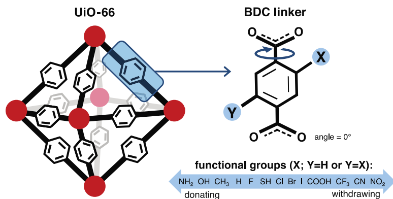
Figure 2. Features of a UiO-66 MOF structure—linker rotation angle, functional group identity, and number of functional groups—studied to observe their effects on methane uptake and diffusion. Red circles represent the UiO-66 secondary building unit (SBU). The angle of rotation of the 1,4-benzenedicarboxylic acid (BDC) linker is with reference to a base configuration (angle=0°) where the benzene is parallel to the carboxyl groups. All linkers are rotated simultaneously by the same angle for each rotamer explored. The identity of the functional groups studied span from electron donating to electron withdrawing. The number of functional groups on each BDC linker is limited to at most 2, where di-functionalized derivatives are placed para to each other.
