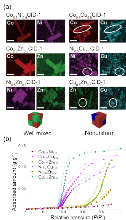
Fig. 4. (a) SEM-EDX maps for \text{M}_{1.0.5}\text{M}_{2.0.5}\text{CID-1} . White circles indicate nonuniform areas. Scale bars: 30 \mu\text{m} . (b) Water-sorption isotherms of \text{M}_{1.0.5}\text{M}_{2.0.5}\text{CID-1} at 298 K. Filled and open symbols correspond to adsorption and desorption, respectively.
