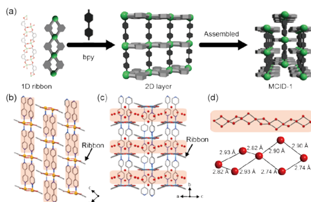
Fig. 1. (a) MCID-1 assembly process. Crystal structures of (b) CoCID-1, (c) CuCID-1·H 2 O, and (d) CuCID-1. The pale-red highlighted regions in (b) and (c) represent pore spaces. The pale-red highlighted region in (c) represents the water chain structure in the 1D channel. Orange, gray, blue, and red represent Co, C, N, and O, respectively. H atoms are omitted for clarity.
