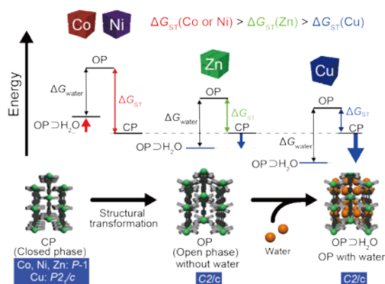
Fig. 3. Proposed energy diagram for the structural transformation. If the \Delta G_{\text{ST}} values for CoCID-1 and NiCID-1 are much larger than proposed, OP \rightarrow H 2 O for CoCID-1 and NiCID-1 will be more unstable than OP for ZnCID-1 and CuCID-1, which cannot be confirmed from the experimental results.
