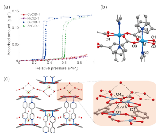
Fig. 2. (a) Adsorption and desorption isotherms for water at 298 K. Filled and open symbols correspond to adsorption and desorption, respectively. Coordination structure of CuCID-1 \rightarrow H 2 O around (b) metal ion and (c) O4 w .
