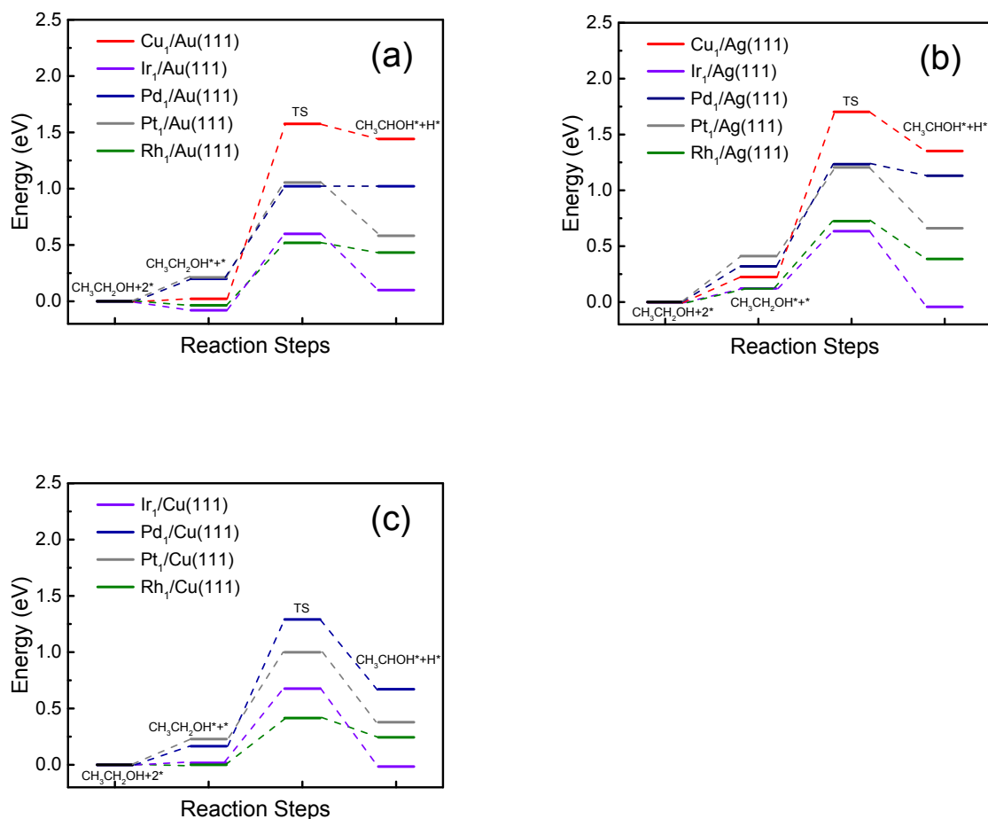
Figure 5. Free energy profiles of \alpha -C-H dehydrogenation selectivity of ethanol on single-atom doped catalysts alloyed into (a) Au(111), (b) Ag(111), and (c) Cu(111).
