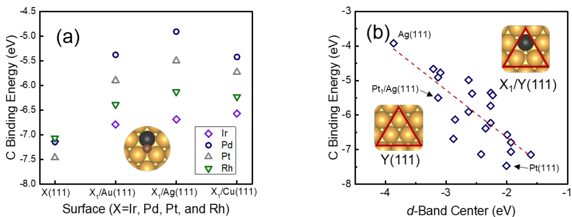
Figure 3. (a) Calculated carbon binding energies on the single-atom alloy surfaces and their monometallic counterparts. Inset shows the binding configuration of carbon at an alloyed triatomic ensemble. (b) Correlation between the carbon binding energies and the calculated d -band centers of the triatomic ensembles. Insets show the triatomic ensembles that considered for the calculations of d -band center. Black, golden, and brown spheres represent X (X=Ir, Pd, Pt, and Rh), Y (Y=Au, Ag, and Cu), and C, respectively.
