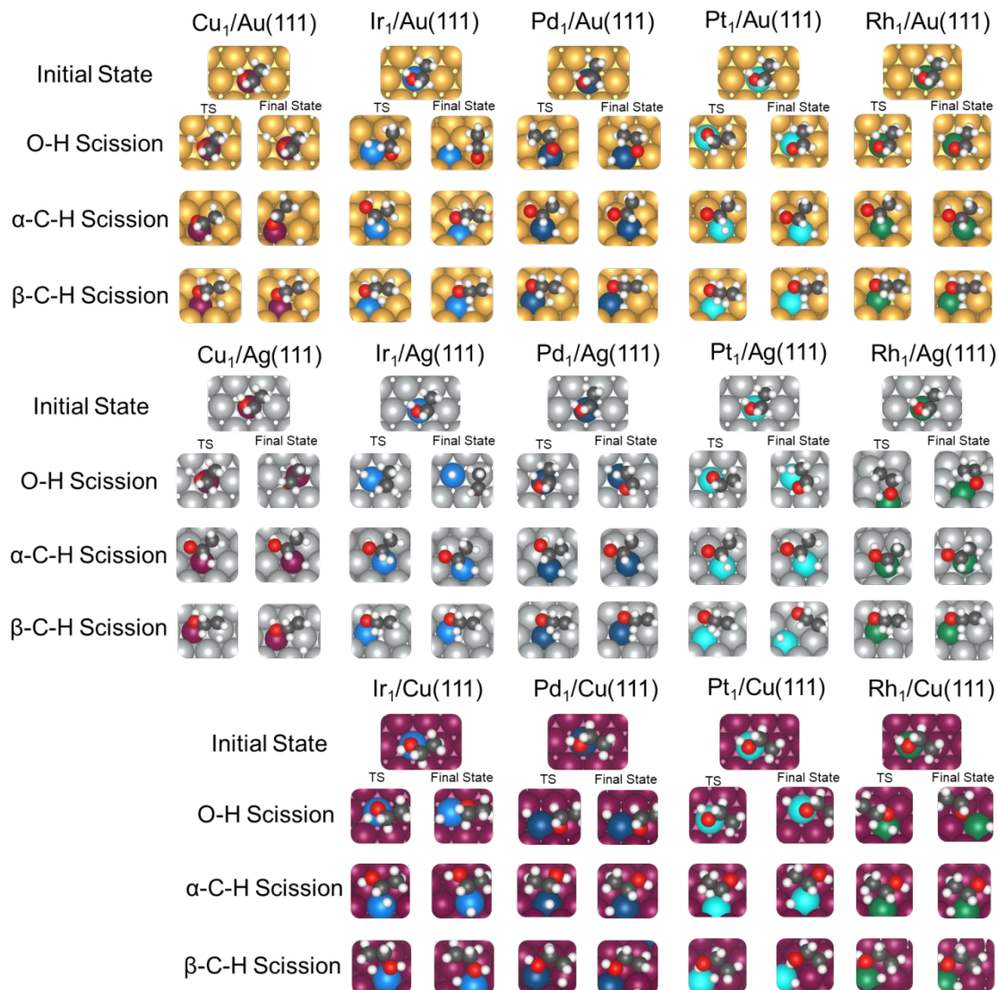
Figure 6. Initial, transition, and final states of EtOH dehydrogenation on X_1/Y(111) ( X =Cu, Ir, Pd, Pt, and Rh; Y =Au, Ag, and Cu) surfaces. Gold, purple, silver, blue, deep blue, teal, green, red, grey, and white spheres represent Au, Cu, Ag, Ir, Pd, Pt, Rh, O, C, and H, respectively.
