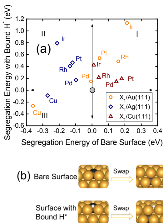
Figure 1. (a) Stability of the single-atom alloy surfaces. X represents the doped single-atom element (Cu, Ir, Pd, Pt, and Rh). (b) Process by which a sublayer element
