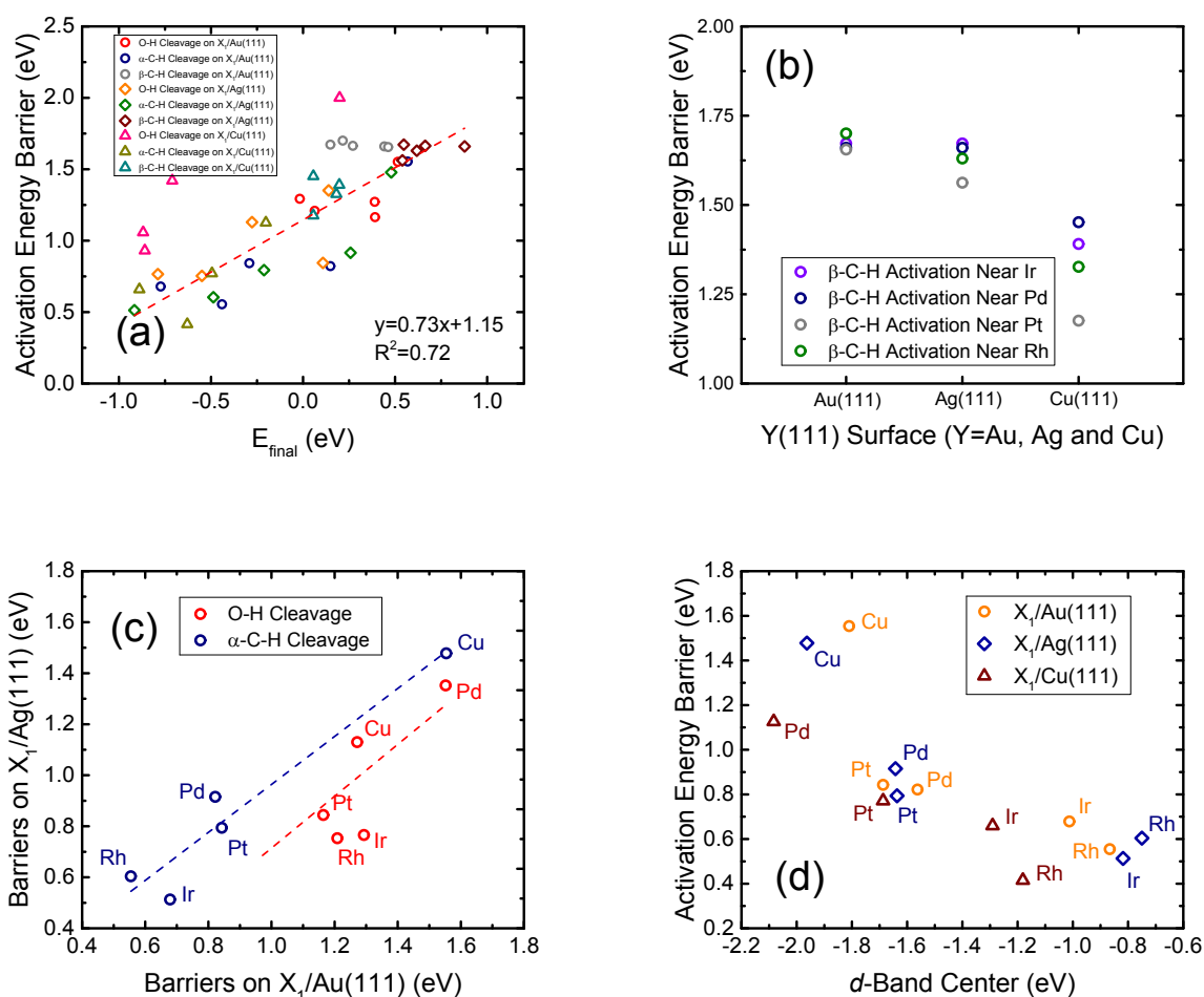
Figure 8. (a) BEP correlation between the activation energy barrier and the final state. E_{\text{final}} are relative to the bare slab and an ethanol (in gas phase). (b) \beta -C-H activation energy vs the three (111) substrates. (c) Correlation on the O-H and \alpha -C-
