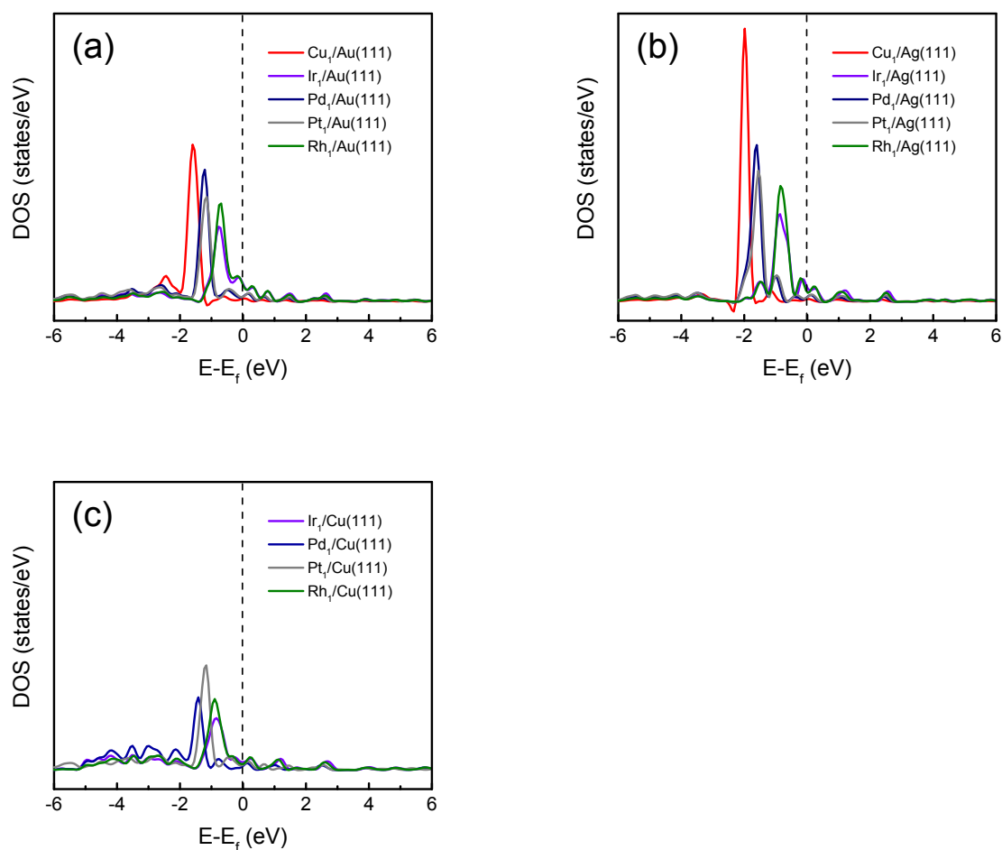
Figure 7. Calculated projected density of states (PDOS) of d -electrons of the single-atom element doped on (a) Au(111), (b) Ag(111), and (c) Cu(111) surfaces. The black dashed lines represent the Fermi energy level ( E_f ).
