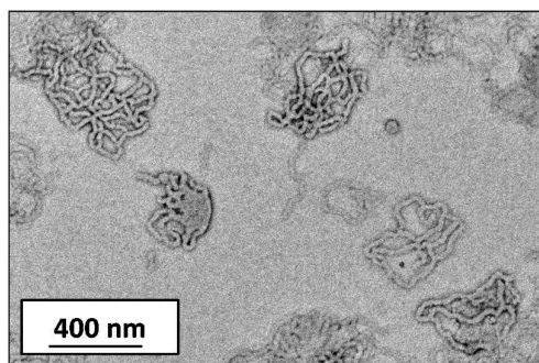
Figure 3 Representative TEM image obtained for the transient 'jellyfish' intermediate structures formed by an MPETTC-PGMA 43 -PHPMA 190 diblock copolymer after 24 h at pH 3.0.
