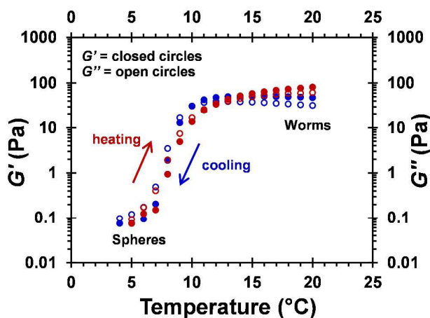
Figure 7 Variation of storage modulus ( G' , filled circles) and loss modulus ( G'' , open circles) with temperature for a 10% w/w aqueous dispersion of MPETTC-PGMA 43 -PPHMA 190 diblock copolymer worms at pH 3. The blue circles represent a cooling cycle from 20 °C to 4 °C and the red circles represent a heating cycle from 4 °C to 20 °C. Measurements were conducted at an angular frequency of 1.0 rad s -1 and an applied strain of 1.0%, with an equilibration time of 20 min at each temperature.
