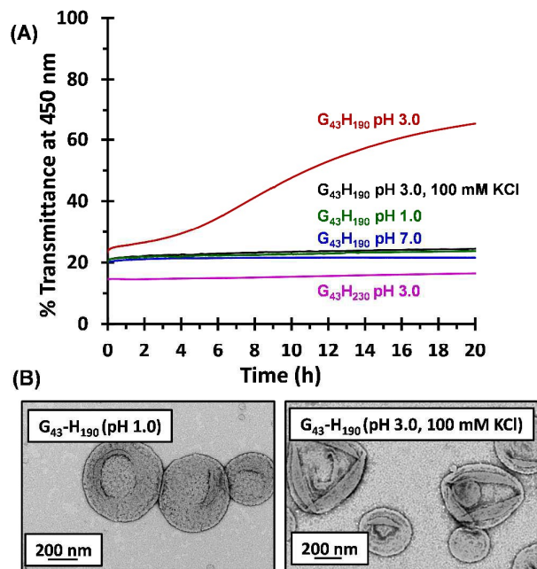
Figure 5 (a) Turbidimetric data obtained for MPETTC-PGMA 43 -PHPMA 190 nano-objects at either pH 7.0, pH 3.0 or pH 1.0, or at pH 3.0 in the presence of 100 mM KCl, for (non-responsive) MPETTC-PGMA 43 -PHPMA 230 vesicles. All measurements were recorded over 20 h for 0.1% w/w dispersions at 20 °C. (b) TEM images obtained for MPETTC-PGMA 43 -PHPMA 190 diblock copolymer vesicles after 20 h at either pH 1.0 in the absence of added salt or pH 3.0 in the presence of 100 mM KCl. This confirms that the original vesicle morphology is retained under these conditions.
