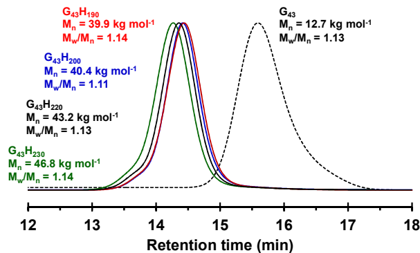
Figure 1 DMF chromatograms obtained for MPETTC-PGMA _{43} macro-CTA (black dotted curve) and the corresponding MPETTC-PGMA _{43} -PHPMA _y diblock copolymer vesicles ( Y = 190, 200, 220 and 230 ). Molecular weight data are calculated relative to a series of near-monodisperse poly(methyl methacrylate) calibration standards. G and H denote poly(glycerol monomethacrylate) and poly(2-hydroxypropyl methacrylate), respectively.
