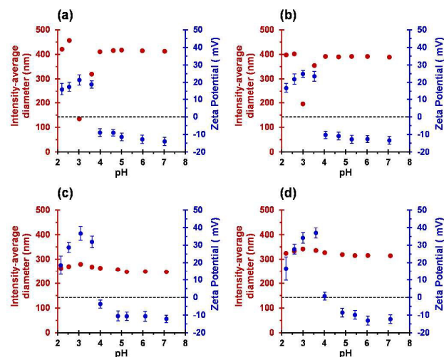
Figure 4 Intensity-average diameter vs. pH and zeta potential vs. pH curves obtained for MPETTC-PGMA 43 -PHPMA γ diblock copolymer nano-objects where \gamma = (a) 190, (b) 200, (c) 220 and (d) 230. All measurements were made at 20 °C for 0.1% w/w copolymer dispersions prepared in the presence of 1 mM KCl background salt.
