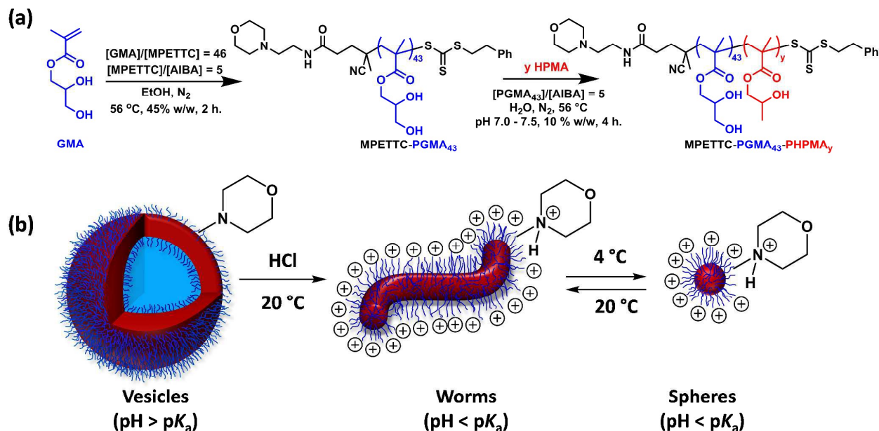
Scheme 1 Schematic representation of (a) the synthesis of MPETTC-PGMA 43 macro-CTA by RAFT solution polymerisation of GMA and its subsequent chain extension with HPMA by RAFT aqueous dispersion polymerisation, at pH 7.0 – 7.5 to prepare PGMA 43 -PHPMA y diblock copolymer vesicles. (b) Schematic cartoon of the vesicle-to-worm transition that occurs when morpholine-functionalised PGMA 43 -PHPMA y diblock copolymer vesicles undergo a pH switch upon addition of acid and the reversible worm-to-sphere transition that occurs upon cooling of these acidified, cationic worms from 20 °C to 4 °C.
