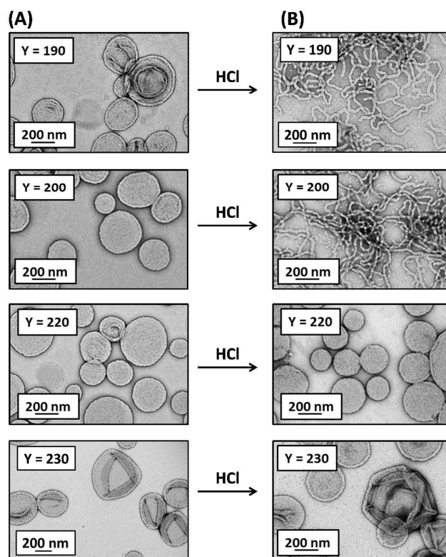
Figure 2 Transmission electron microscopy images obtained for 0.1% w/w aqueous dispersions of MPETTC-PGMA _{43} -PHPMA _y ( y = 190, 200, 220 and 230 ) diblock copolymer nanoparticles at either (A) pH 7.0 or (B) pH 3.0. The pH switch was performed at 20 ^{\circ}\text{C} at 10% w/w copolymer concentration in each case.
