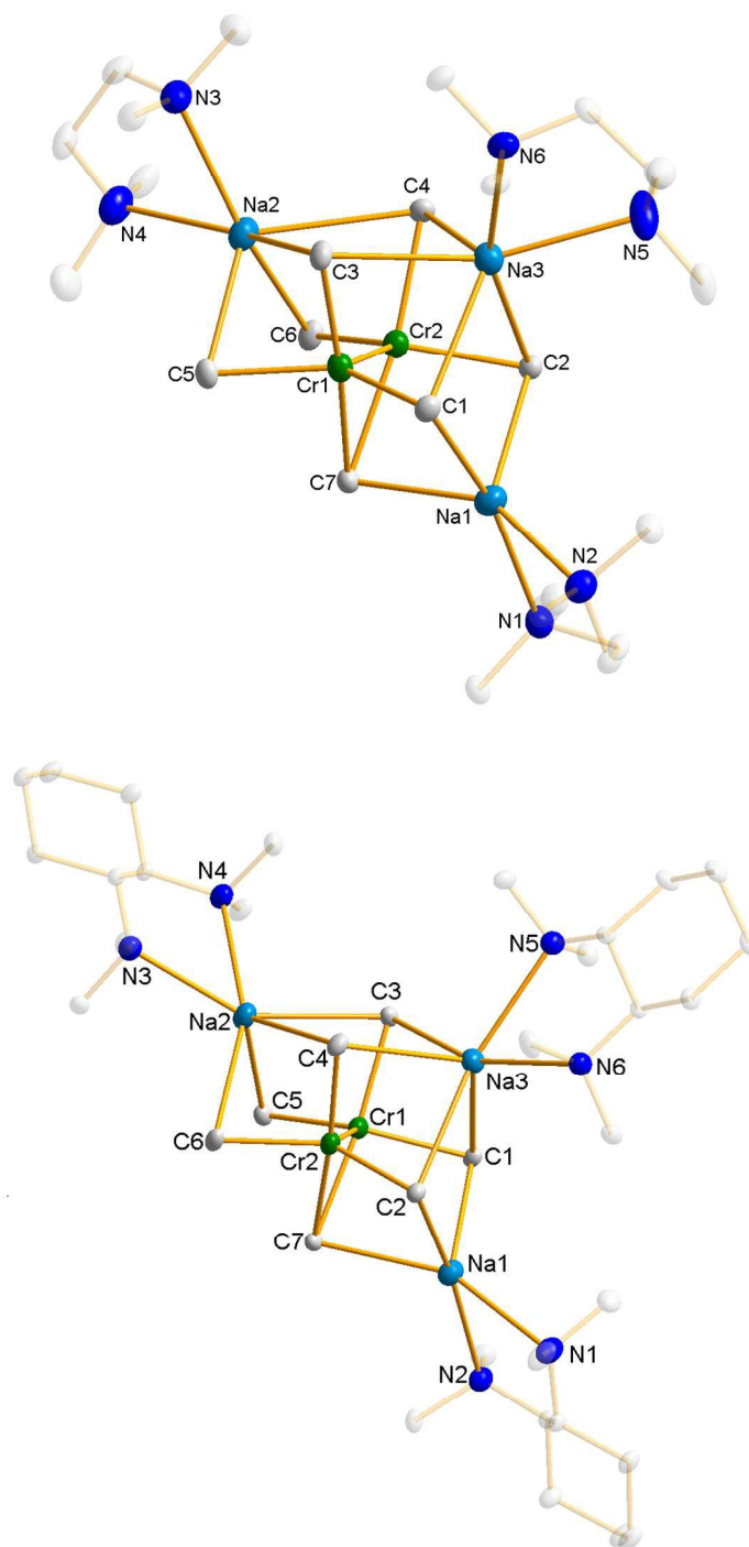
Figure 2. Molecular structure of [(\text{TMEDA})\text{Na}]_3\text{Cr}_2\text{Me}_7 ( 6 , top) and [(\text{TMCDA})\text{Na}]_3\text{Cr}_2\text{Me}_7 ( 7 , bottom) with hydrogen atoms and minor disorder of one TMEDA ligand of 6 omitted for clarity. Thermal ellipsoids are represented at 50% probability.
