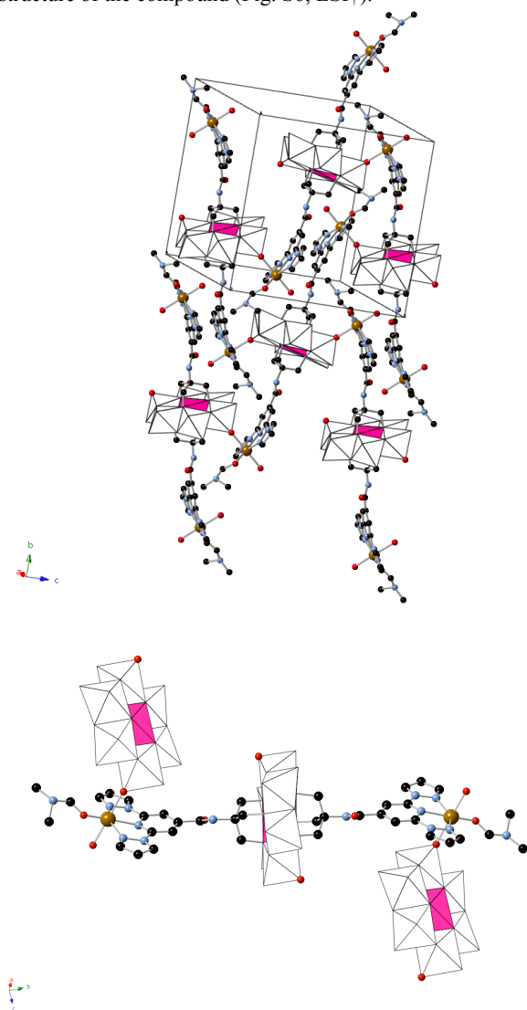
Fig. 2 Views of a layer of functionalized-POM linked through \text{Fe}^{2+} ions in the structure of 2 (top) and of the repeating trimeric unit with two coordinated POMs (bottom) (Fe (yellow), Mn (pink), Mo (white), C (black), N (blue), O (red)). Red oxygen atoms from the POM are those coordinated to \text{Fe}^{2+} ions. Hydrogen atoms have been omitted for clarity.
