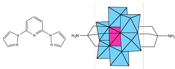
Scheme 1 Molecular structure of 1-bpp (left) and 4 (right).
