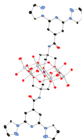
Fig. 1 View of the structure of the functionalized-POM in compound 1 . (Mn (pink), Mo (white), C (black), N (blue), O (red)). Hydrogen atoms have been omitted for clarity.
