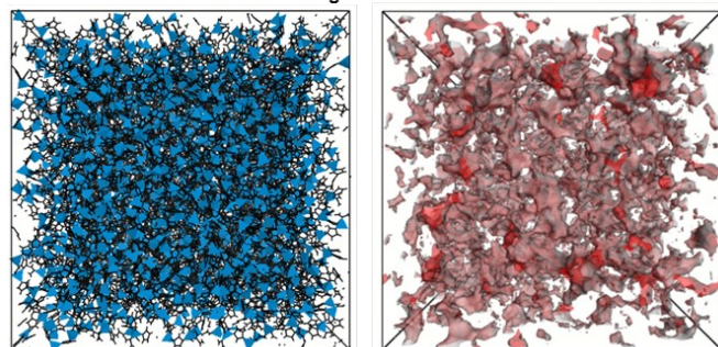
Figure 1. Structures for ZIF-4 (4x4x4 supercell, CCDC 602538), ZIF-zni (4x4x4 supercell, CCDC 120379) and a_g ZIF-4 (2062 Zn atoms). Left: Atomic structures with ligands in black and zinc in blue. Right: Accessible porosity shown as a red Connolly surface, using a probe of 1 Å in diameter.
