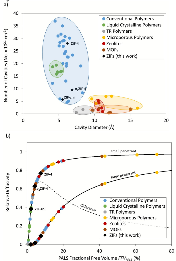
Figure 4. a) Comparison of PALS results for a range of materials including polymers, zeolites, MOFs and the present study of ZIF glasses. Only the cavity diameters for the fourth component ( \tau_4 ) are displayed where multi-modal distributions exist. b) Relative diffusivity predicted from Cohen and Turnbull equation with arbitrary penetrant radii of 0.6 and 1.4 Å. References in Table SI-2.
