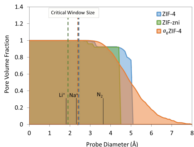
Figure 3. Pore volume fraction calculated for ZIF-4, ZIF-zni and a g ZIF-4 with a range of probe diameters. Dashed lines represent the critical window size for free transport according to the Voronoi representation using Zeo++ . 24,25 Note that ZIF-4 undergoes a pressure-induced phase transition, which is not reflected in this scheme.
