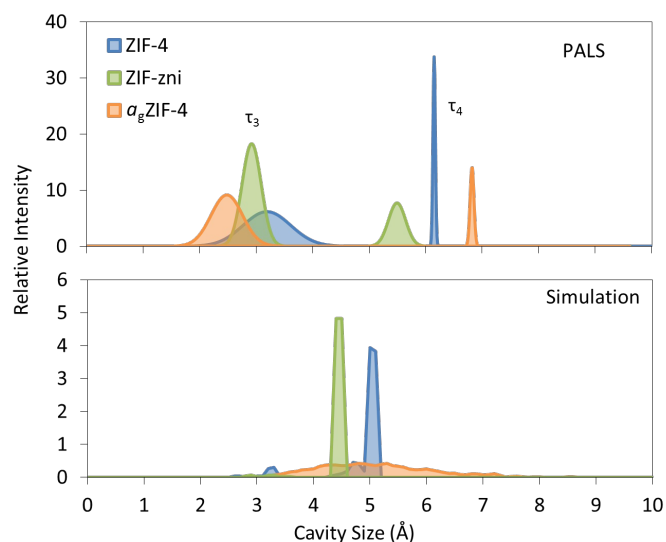
Figure 2. Pore size distributions measured with PALS and simulated with Zeo++ 24,25 for ZIF-4, ZIF-zni and a_g ZIF-4. PALS results for the third and fourth components ( \tau_3 and \tau_4 ) are represented as Gaussian distributions which correspond to the small and large cavities, respectively.
