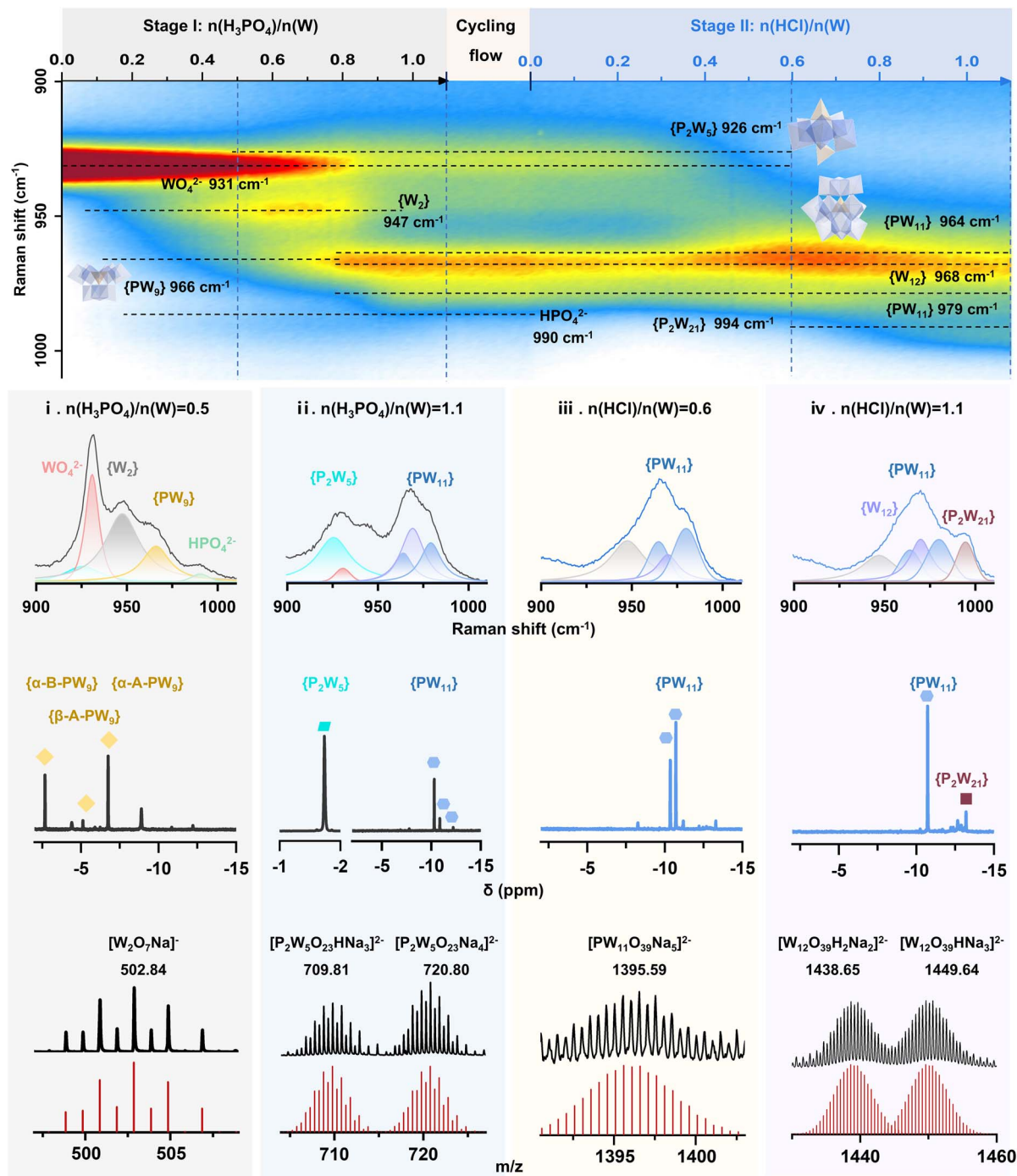
Fig. 2 Stage I–II of the acid titration process: the time-dependent 2D Raman mapping (900 cm −1 to 1010 cm −1 ), along with corresponding Raman spectra, 31 P NMR spectra and ESI-MS spectra in the negative ion mode (the red and black lines represented simulated and experimental values, respectively) at different n(\text{H}_3\text{PO}_4)/n(\text{W}) ratios or n(\text{HCl})/n(\text{W}) ratios. Stage I and stage II were separated by a cycling flow, which showed that the Raman signal remained unchanged during this interval.
