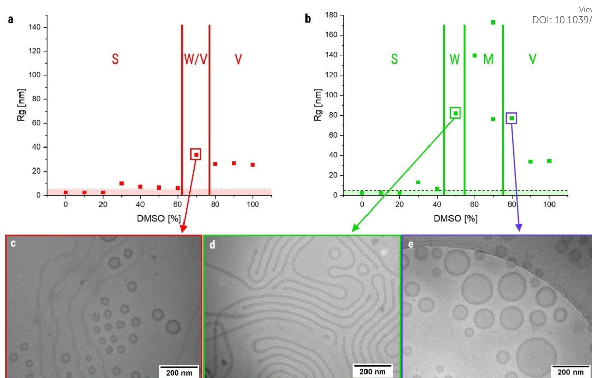
Figure 4: Morphological investigations about the influence of initial polymer concentration. R_g over DMSO ratio which was used for solvent switch procedure with initial polymer concentration of a) 1 mg/mL and b) 7 mg/mL. Water addition rate was kept at 2 mL/h. Morphologies were assigned to values based on particle size and cryo-TEM images. S = spheres, W = worm-like micelles, V = vesicles, M = mixed morphologies. Cryo-TEM images of c) 1 mg/mL, 70% DMSO (worm-like micelles and small vesicles); d) 7 mg/mL, 50% DMSO (predominantly worm-like micelles); e) 7 mg/mL, 80% DMSO (vesicles).
