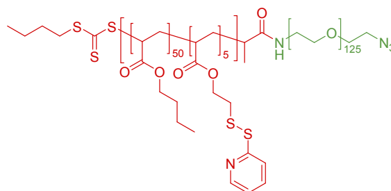
Figure 1: Chemical structure of the amphiphilic block copolymer P(BA 50 -PDSA 5 )- b -PEO 125 -N 3 used for nanoparticle formation.
