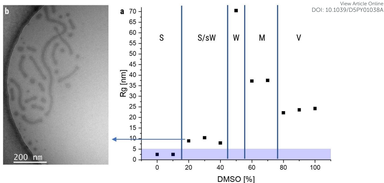
Figure 6: a) R_g over DMSO content which was used for solvent switch procedure for an initial polymer concentration of 4 mg/mL and a water addition rate of 20 mL/h. Morphologies were assigned to values based on particle size and cryo-TEM images. S = spheres, sW = small worm-like micelles, W = worm-like micelles, M = mixed morphologies, V = vesicles; b) Cryo-TEM image for 20% DMSO showing short worm-like micelles besides spherical micelles.
