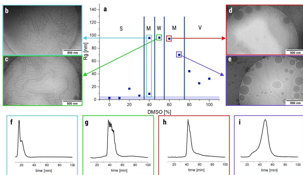
Figure 3: Morphological investigations of samples prepared from different starting solvent compositions with increasing DMSO content (100% acetone to 100% DMSO) by AF4 and cryo-TEM. The concentration and water addition rate were kept at 4 mg/mL and 2 mL/h, respectively. S = spheres, M = mixed morphologies, W = worm-like micelles, V = vesicles. The a) R_g over solvent ratio. Morphologies were assigned to values based on particle size and microscopy images. b) Spherical and worm-like micelles at 40% DMSO; c) worm-like micelles at 50% DMSO; d) worm-like micelles and a small amount of vesicles at 60% DMSO; e) vesicles and a small amount of worm-like micelles at 70% DMSO; AF4 elugrams measured with UV detector at 280 nm for f) 40%; g) 50%; h) 60% and i) 70% DMSO.
