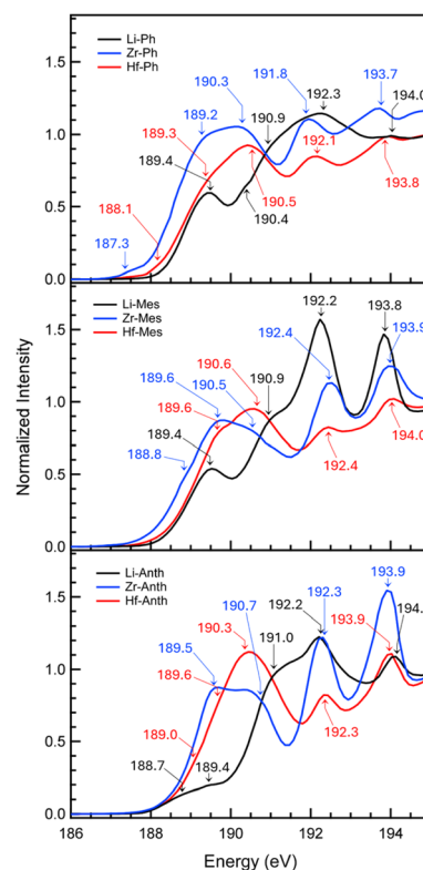
Fig. 7 B K-edge XAS spectra of [\text{M}(\text{RBH}_3)_4] complexes with \text{M} = \text{Zr} (blue) and \text{Hf} (red) and comparison to their corresponding \text{Li}(\text{RBH}_3) salts (black). Labeled positions indicate peak maxima in the spectra or peak positions identified by analysis of the second derivative traces (Fig. S51–S53; SI).
