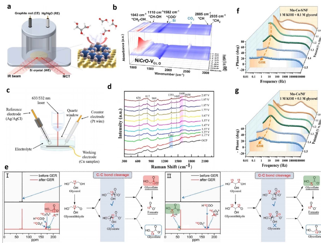
Fig. 5 (a) Illustration of in situ ATR-SEIRAS. (b) In situ ATR-SEIRAS spectra of the GOR on \text{NiCrO-V-Cr}_2\text{O}_3 nanosheet electrodes at various potentials. Reproduced from ref. 63, copyright 2024, American Chemical Society. (c) Schematic diagram for in situ Raman measurements. (d) In situ electrochemical Raman spectra on Cu NPs in 0.1\text{ M KOH} with 0.1\text{ M} glycerol solution. Reproduced from ref. 70, copyright 2023, Elsevier. (e) ^{13}\text{C} -NMR spectra for the electrooxidation of isotope-labelling (I) 2\text{-}^{13}\text{C} glycerol and (II) 1,3\text{-}^{13}\text{C} glycerol. Reproduced from ref. 60, copyright 2023, Elsevier. Bode plots of \text{Mn-Co-S/NF} (f) and \text{Mn-Co/NF} (g) for the GOR. Reproduced with permission from ref. 66, copyright 2024, Elsevier.
