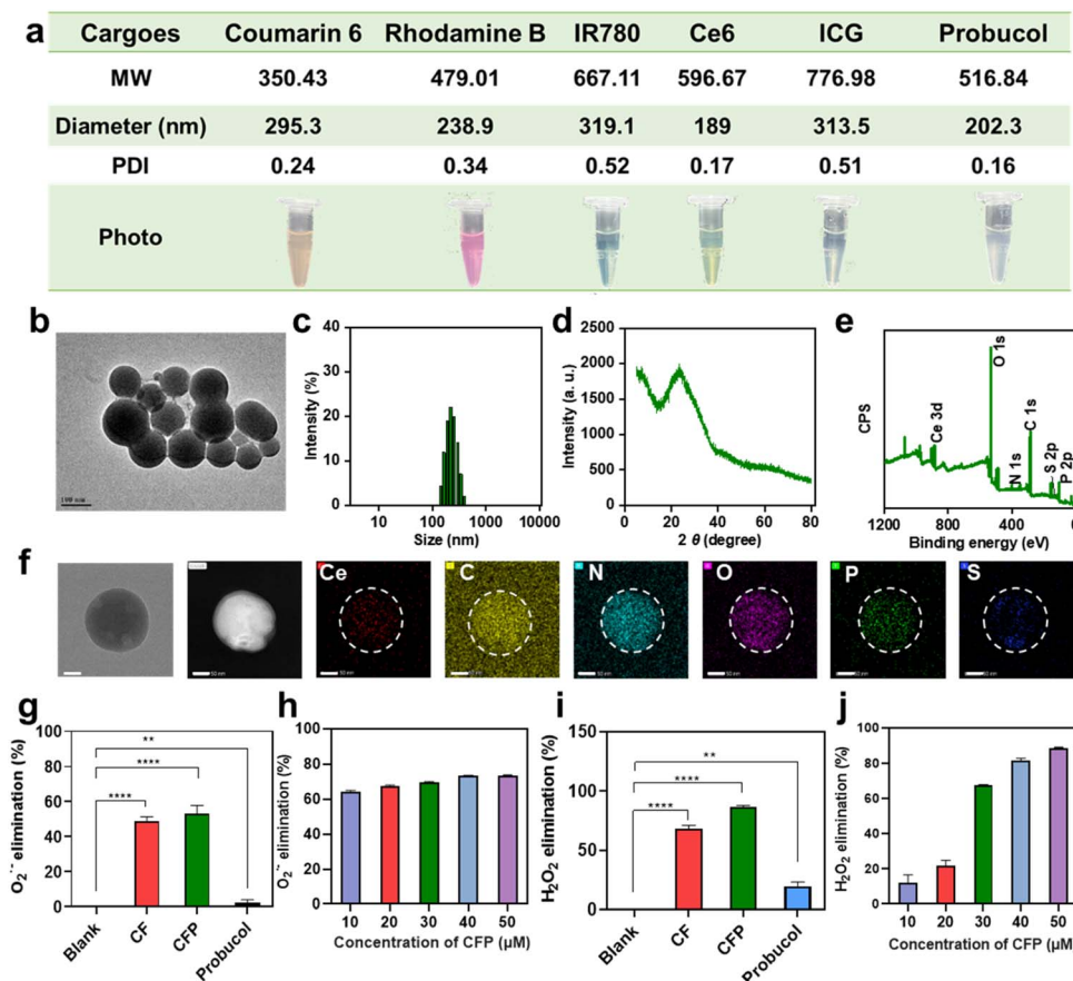
Fig. 2 Moonlighting protein-like multi-functions of CF nanoassembly. (a) CF as a nanocarrier for the loading of different cargos (Coumarin 6, Rhodamine B, IR780, Ce6, ICG, and probuol). (b) TEM image of CFP, scale bar: 100 nm. (c) Hydrodynamic diameter of CFP. (d) XRD pattern of CFP. (e) XPS survey spectrum of CFP. (f) EDS elemental mapping images of CFP. Scale bar: 50 nm. (g) O_2^{\cdot-} -eliminating capabilities of CF, CFP and probuol. (h) CFP concentration-dependent O_2^{\cdot-} -eliminating capability. CFP concentration is represented as Ce concentration. (i) H_2O_2 -eliminating capabilities of CF, CFP and probuol. (j) CFP concentration-dependent H_2O_2 -eliminating capability. CFP concentration is represented as Ce concentration.
