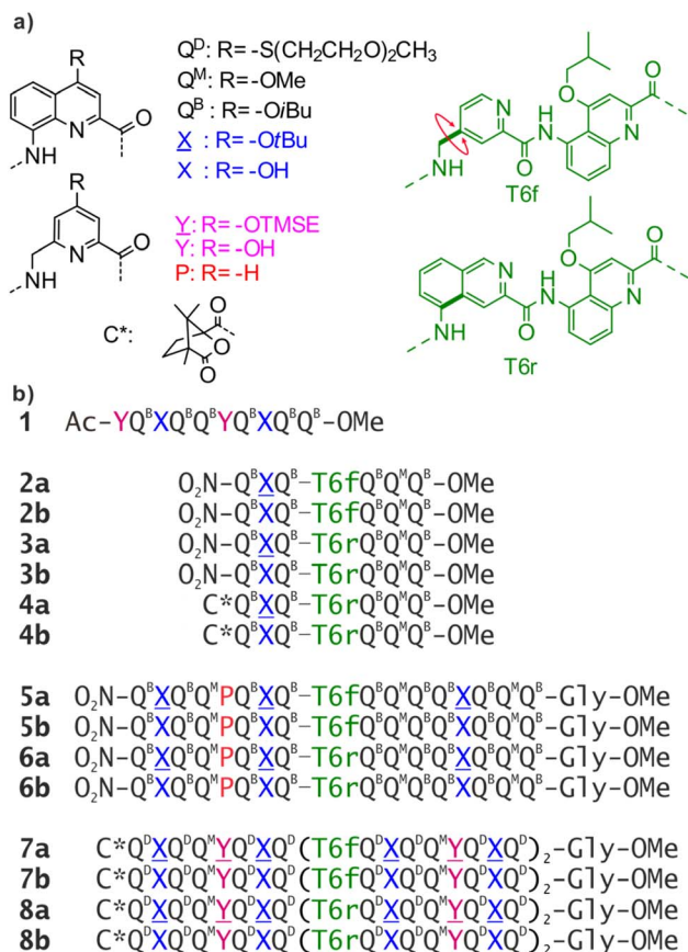
Fig. 1 (a) Structure of Q^D , Q^B , Q^M , X , Y , P , T6f, and T6r monomers as well as N-terminal chiral C^* group. X and Y are the hydroxy protected precursors of X and Y , respectively. TMSE = 2-trimethylsilyl-ethyl. (b) Oligoamide foldamer sequences. The Gly at the C terminus stands for glycine. In sequences ending with an 8-nitro group, this group replaces the terminal amine.
