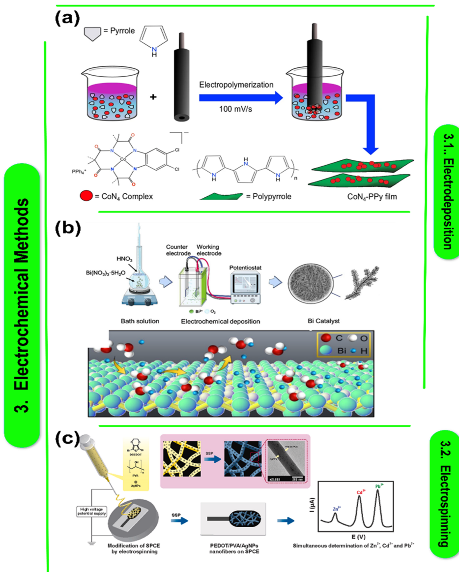
Fig. 2 (a) Diagram showing the electrochemical deposition of PPy sheets using the pyrrole and CoN 4 combination. An electrode made of glassy carbon (GCE) was used for the deposition process. The Co metal's elemental composition, bond formation, and oxidation state in the thin film were examined using X-ray photoelectron spectroscopy (XPS). 65 This figure has been reproduced from ref. 65 with permission from Nature Publishing Group, copyright 2019. (b) Diagram of the constant current two-electrode bismuth electrodeposition device. 66 This figure has been reproduced from ref. 66 with permission from Nature Publishing Group, copyright 2022. (c) Diagrammatic illustration of solid-state polymerized poly(3,4-ethylenedioxythiophene) conductivity-based electrospun nanocomposite fibers that enable simultaneous electrochemical metal ion detection. 68 This figure has been reproduced from ref. 68 with permission from Elsevier, copyright 2022.
