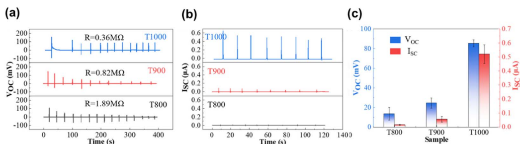
Fig. 22 (a) Measured open circuit voltage ( V_{\text{OC}} ) and (b) short circuit current ( I_{\text{SC}} ) for Magnéli phase nanocrystal films prepared at different temperatures (800–1000 ^\circ\text{C} ) and (c) average peak values of V_{\text{OC}} and I_{\text{SC}} . Reprinted with permission from ref. 129. Copyright 2021, American Chemical Society.
