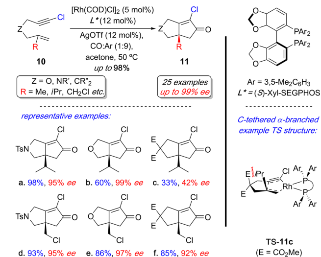
Scheme 9 Overview of Rh(I)-catalyzed enantioselective PKR with 1,6-chloroenynes with representative examples.
