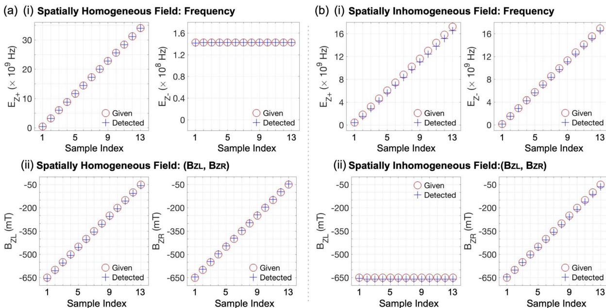
Fig. 5 (a) Performance of the DQD sensing protocol when the sensing target is constant (spatially homogeneous). Being secured with B_{ZL(External)} (=B_{ZL} = B_{ZR}) that varies from -650 mT to -50 mT with an incremental step of 50 mT, simulation results well confirm the operational feasibility of the sensing protocol, so the inaccuracies of E_{Z+} 's & E_{Z-} 's derived from simulated |\psi_M\rangle are just 0.49 \pm 0.83\% & 0.090 \pm 0.21\% of their theoretical values, and, accordingly, the detected B_{ZL} 's & B_{ZR} 's deviate by -5.72 \pm 0.47 mT and 4.49 \pm 0.46 mT from their given quantities, respectively. (b) Computational results driven with spatially inhomogeneous B_{Z(External)} that is considered with B_{ZL} = -650 mV and B_{ZR} varying from -650 mT to -50 mT with a step of 50 mV. As similarly to the case of homogeneous targets, detected values here solidly follow given quantities. While the accuracies generally become worse than the case of homogeneous targets ( E_{Z+} 's: 6.70 \pm 3.81\% , E_{Z-} 's: 2.20 \pm 0.41\% , B_{ZL} 's: -10.02 \pm 1.35 mT, and B_{ZR} 's: -7.00 \pm 5.27 mT), simulation results are fair enough to claim the operational feasibility of the protocol under inhomogeneous sensing targets.
