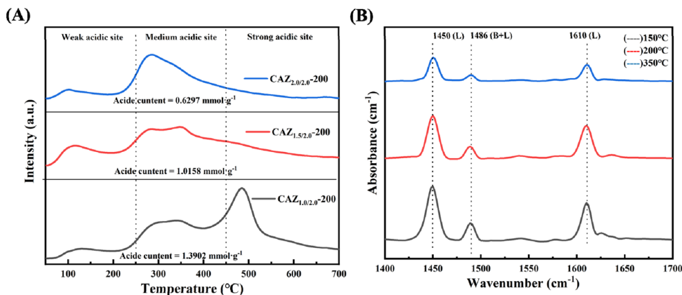
Fig. 4 (A) NH 3 -TPD of the catalyst CAZ 1.0/2.0 -200, CAZ 1.5/2.0 -200 and CAZ 2.0/2.0 -200, (B) Py-IR of the catalyst CAZ 1.5/2.0 -200 at different test temperatures.
