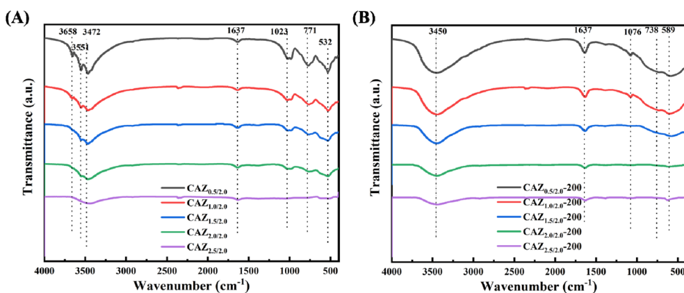
Fig. 5 FT-IR spectra of (A) CAZ x/2.0 precursor and (B) CAZ x/2.0 -200 catalysts.
