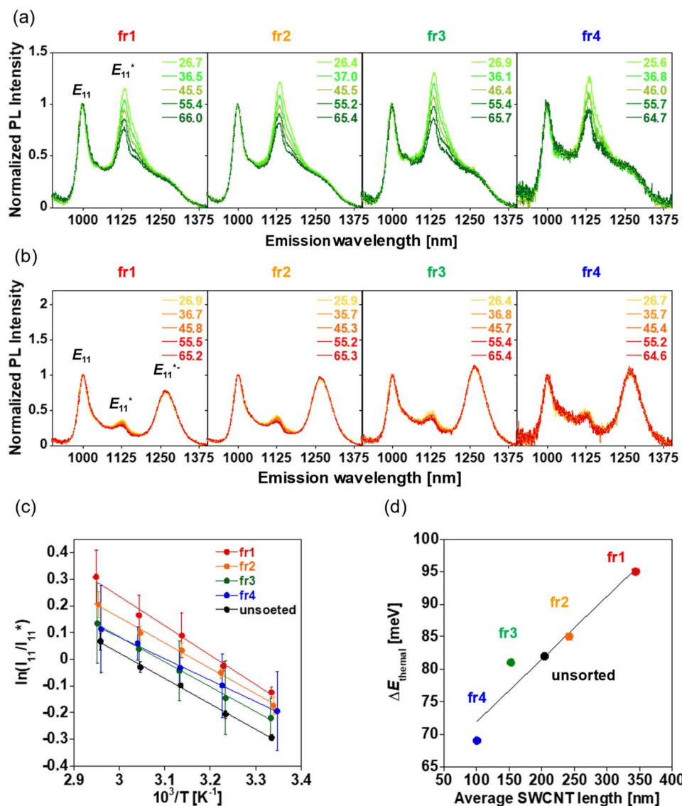
Fig. 7 Temperature-dependent PL spectra (excitation: 570 nm) of the length-sorted (a) gel-coated If-SWCNTs- p\text{NO}_2 solution and (b) gel-coated If-SWCNTs-oP solution in \text{H}_2\text{O} , (c) the van't Hoff plot of the length-sorted and unsorted gel-coated If-SWCNTs- p\text{NO}_2 solution, and (d) plot of \Delta E_{\text{thermal}} as a function of the average SWCNT length. Error bars mean the error estimated during peak deconvolution.
