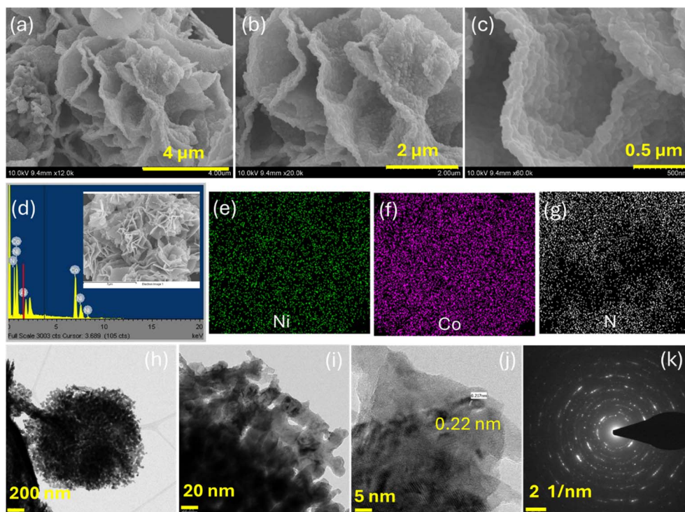
Fig. 3 (a–c) SEM, (d) EDS spectrum, (e–g) EDS mapping images, (h) TEM, (j) HR-TEM, and (k) SAED pattern of as-prepared NiCoN electrode.
