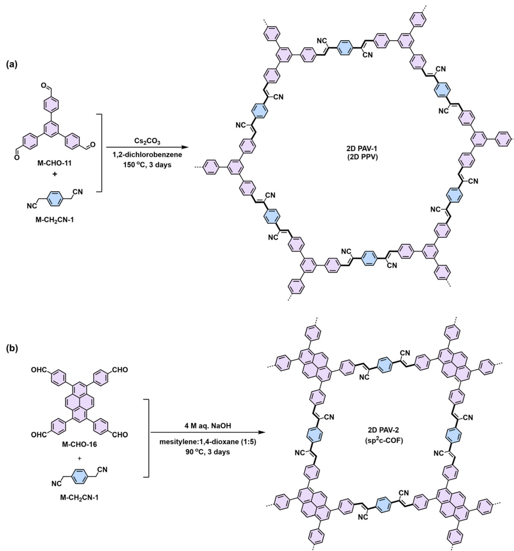
Scheme 4 Synthesis of (a) 2D PAV-1 (2D PPV) with hexagonal lattice and (b) 2D PAV-2 ( \text{sp}^2\text{c-COF} ) with 2D square lattice.
