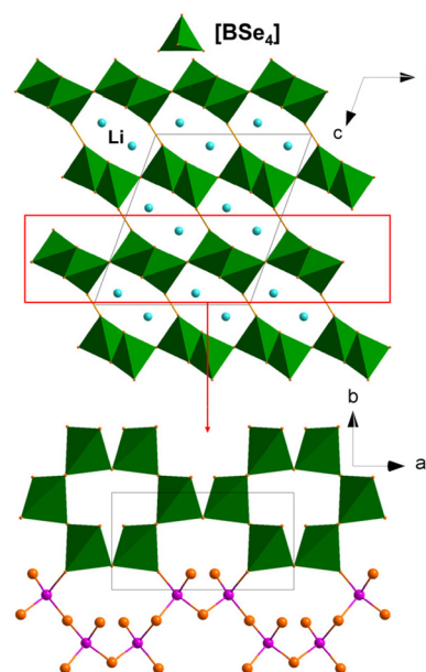
Fig. 11 The structure of \text{Li}_2\text{B}_2\text{Se}_5 .
