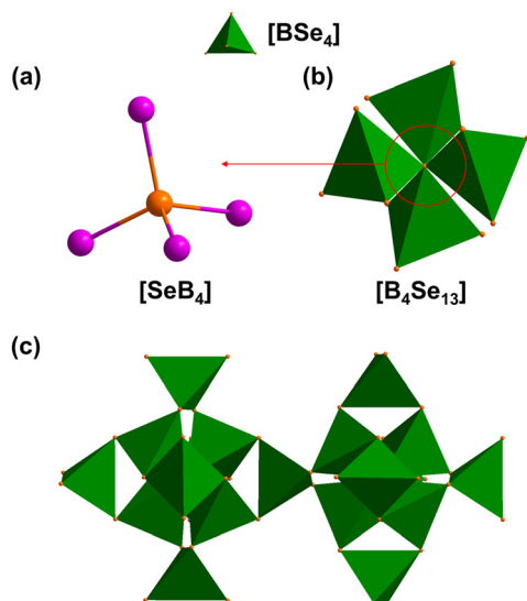
Fig. 10 Basic building block of the \text{B}_7\text{Se}_{13}^{5-} anion in \text{Li}_7\text{B}_7\text{Se}_{15} . (a) \text{SeB}_4 tetrahedron forming (b) \text{B}_4\text{Se}_{13} basic units interconnected via additional BSe units to (c) \text{B}_7\text{Se}_{13}^{5-} entities forming the network.
